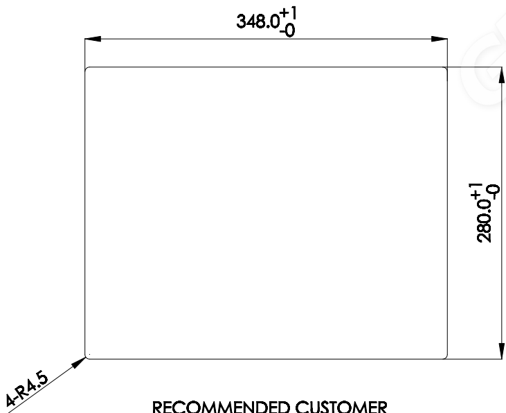
RECOMMENDED CUSTOMER PANEL CUT-OUT
