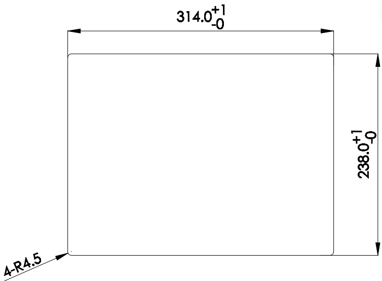
RECOMMENDED CUSTOMER PANEL CUT-OUT
