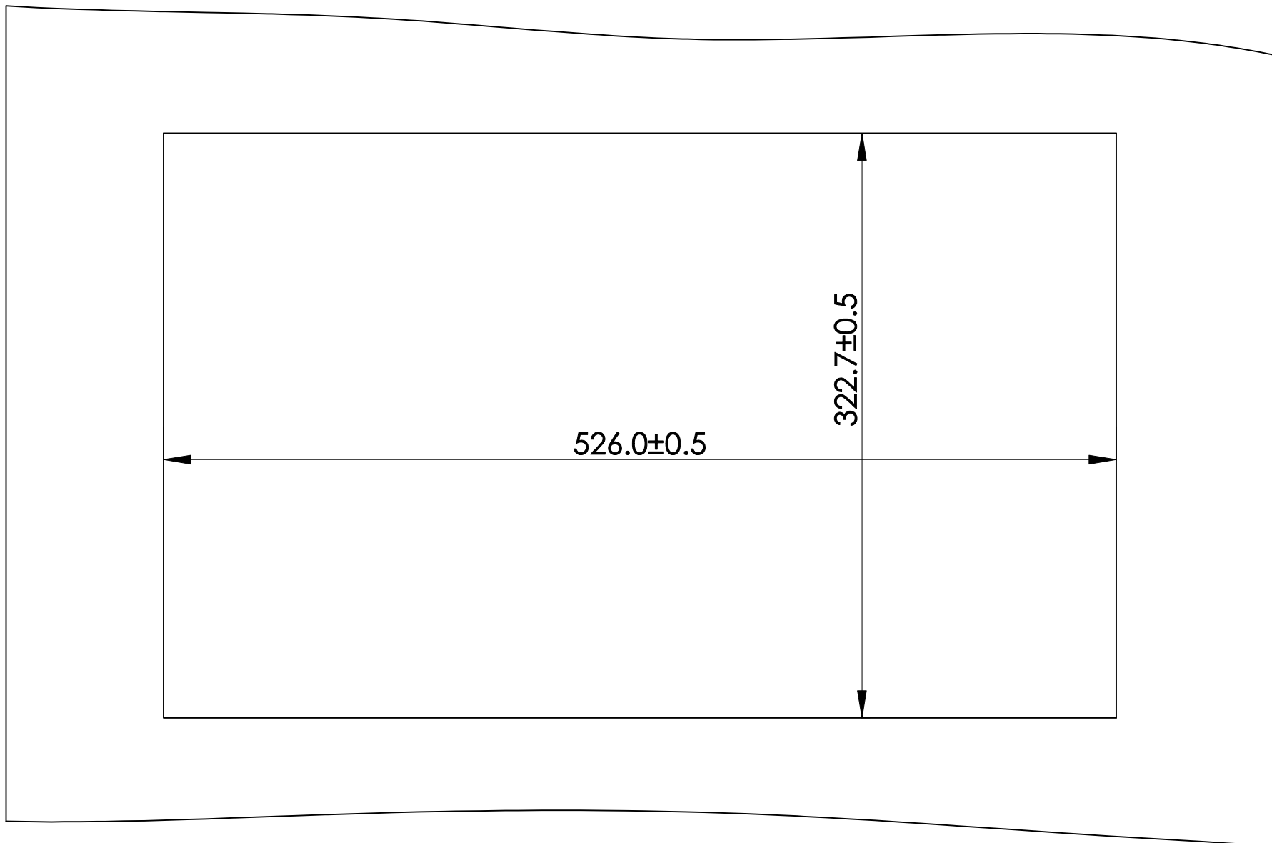
RECOMMENDED OPENING SIZE OF CABINET DOOR PANEL
