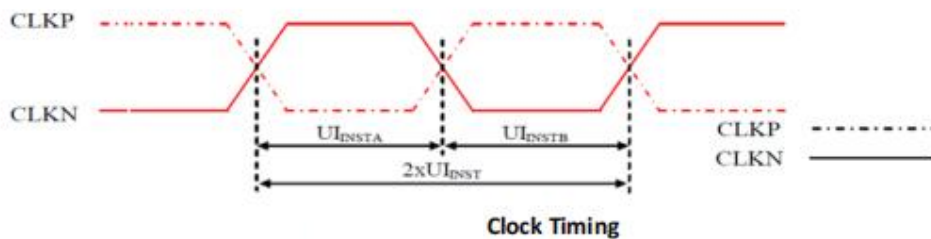
High Speed Mode - Clock / Data Timings
