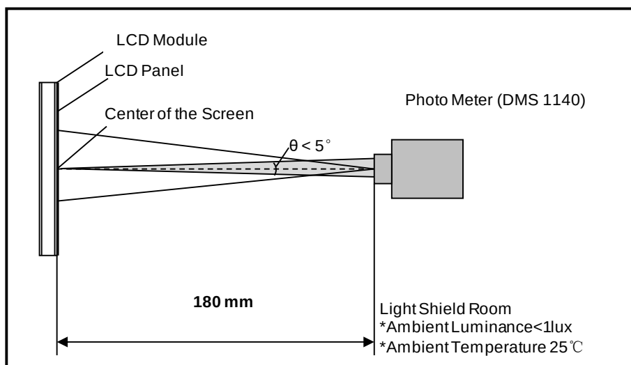
Figure 3 Measurement Setup
