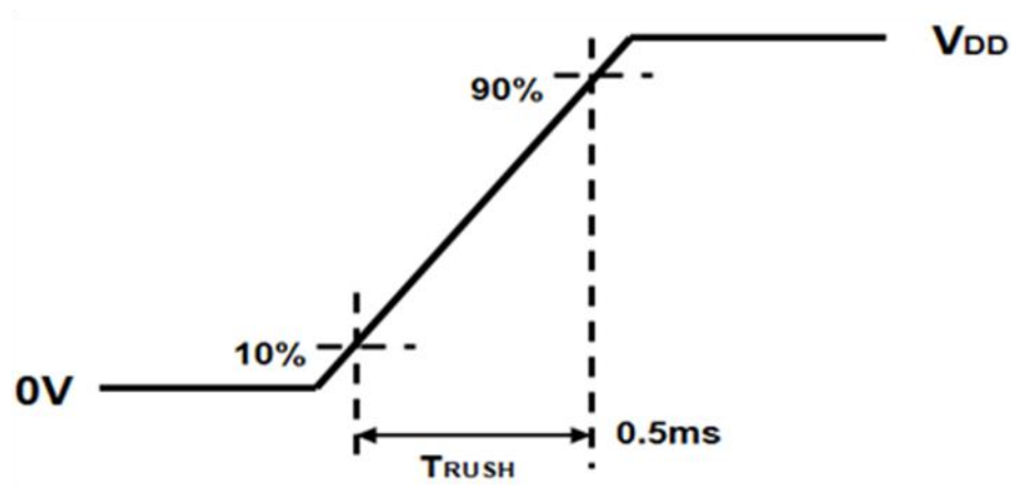
Figure 3 V_{DD} Rising Time
