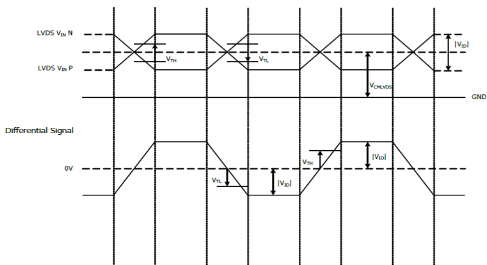
Figure 7 Voltage Definitions
