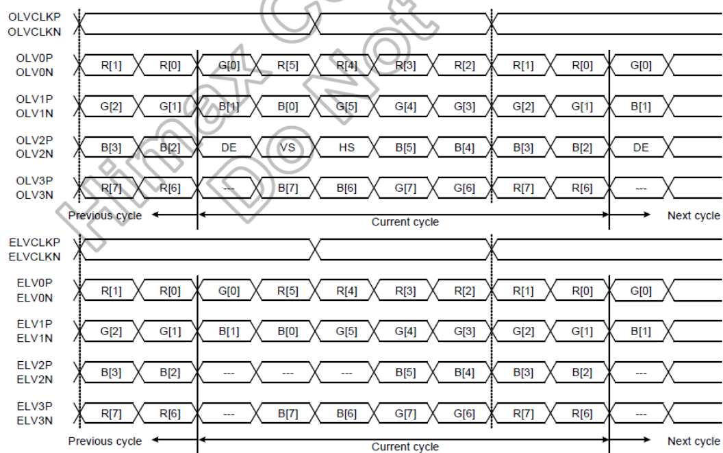
Figure 8 Data Mapping
