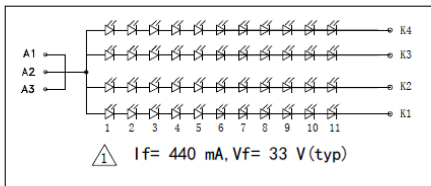
NTC CIRCUIT DIAGRAM
