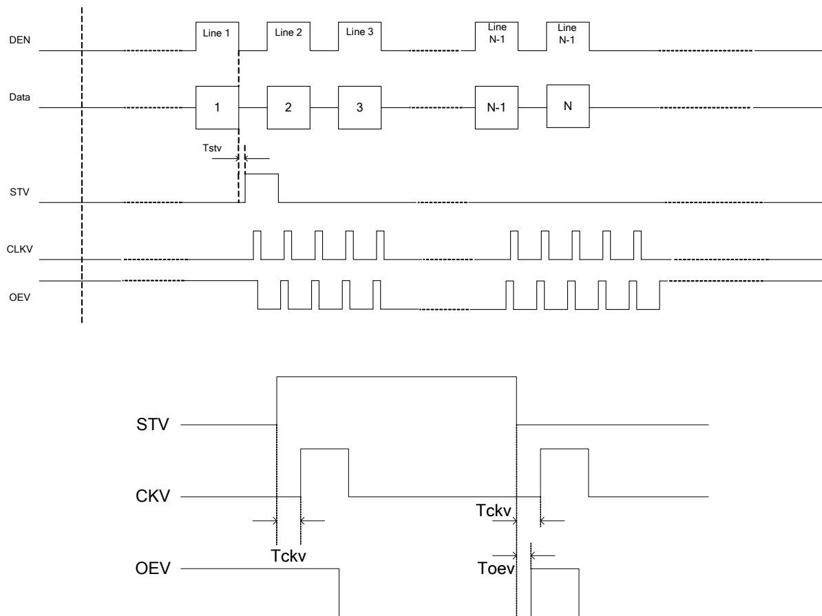
Vertical Timing Diagram DE
