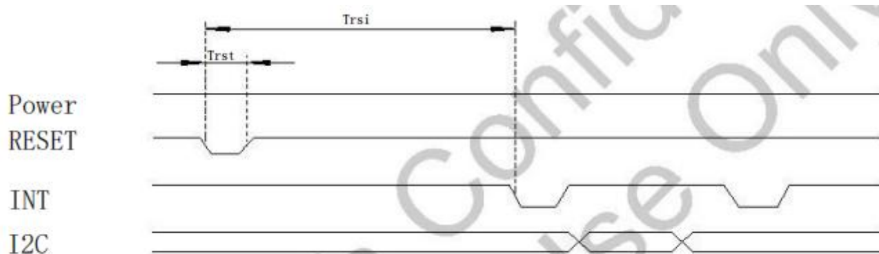
Figure 3-6 Reset Sequence
