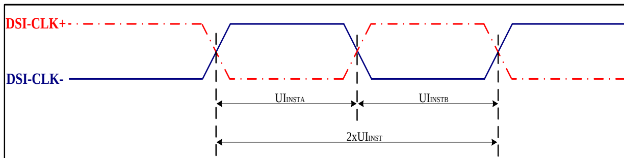
Figure DSI clock channel timing
