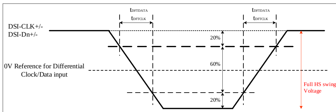
Figure Rising and falling time on clock and data channel
