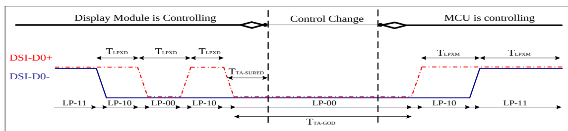
Figure BTA from Display Module to MCU Timing
