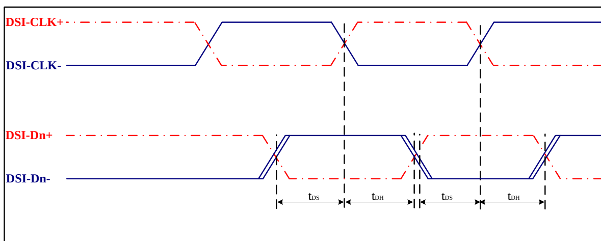
Figure 6-5-3-1-2 DSI data to clock channel timing
