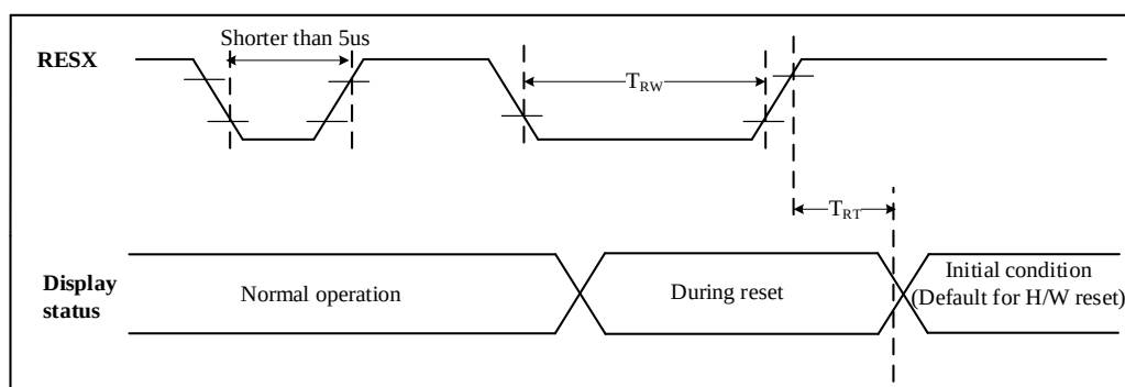
Figure 6-5-4 Reset Timing
