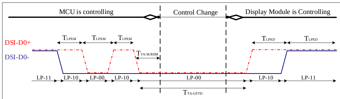
Figure BTA from MCU to Display Module Timing
