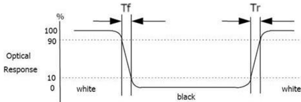
<Figure . Response Time Testing>
