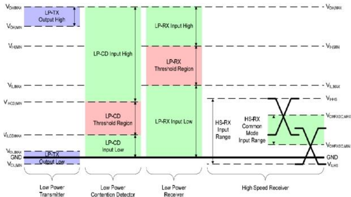
Figure MIPI DC Timing Characteristics
